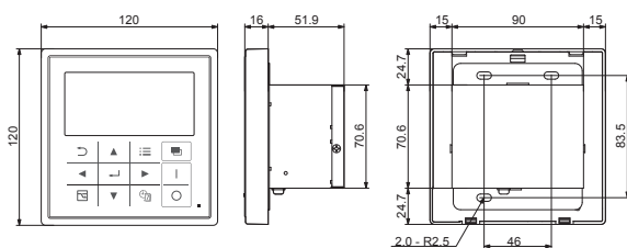
System Controller
