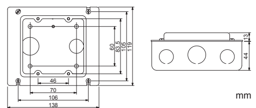
Switch Box
