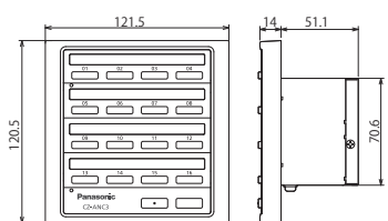
ON/OFF Controller
