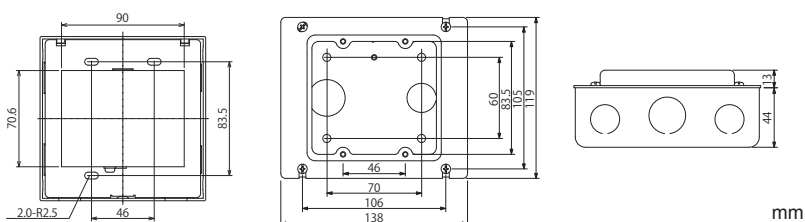
Switch box
